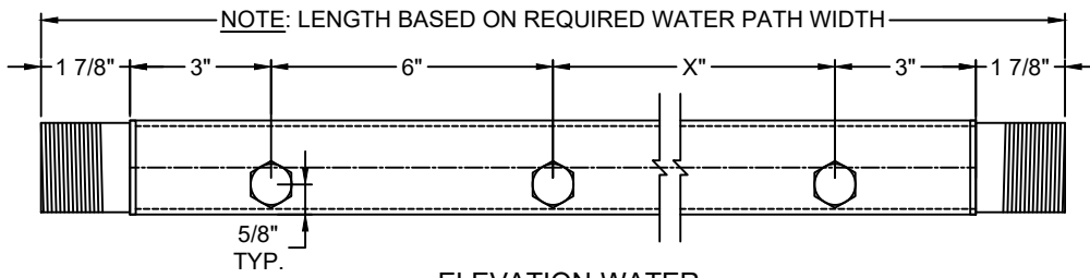
ELEVATION-WATER DELIVERY SIDE
